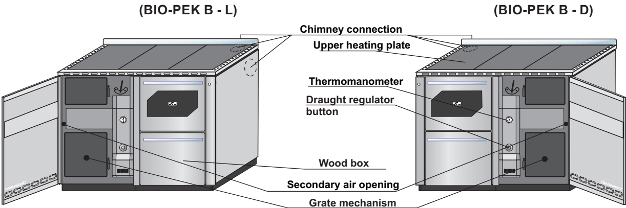
Image 9. Basic parts
